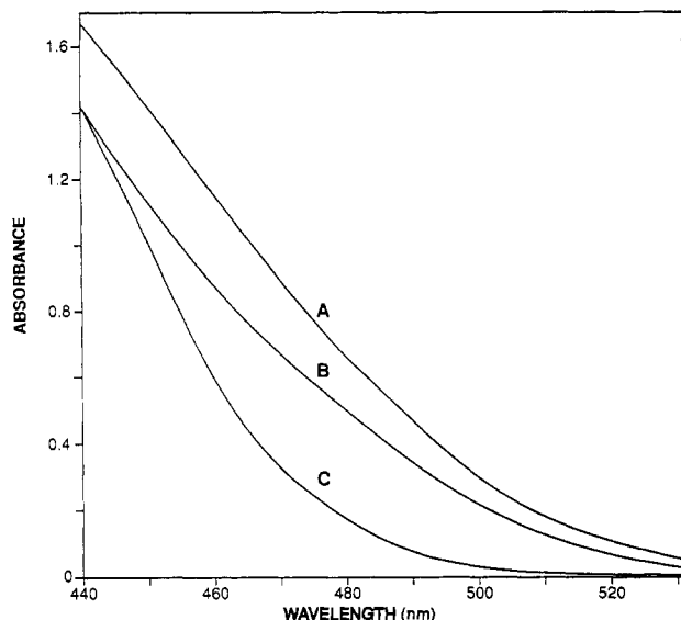
Figure 3. Spectra derived from rapid-scan measurements (440–540 nm, path length 2.0 cm) following ratio mixing (1:14.4) of 5.555 \times 10^{-2} M Cr(VI) (pH 3.5) with 0.50 M TRIS buffer ( I = 1.0 M ( \text{NaClO}_4 ), [\text{Cr(VI)}]_{\text{T}} = 3.607 \times 10^{-3} M, 25^\circ\text{C} , pH 8.8). Spectra correspond to the following: (A) 1.803 \times 10^{-3} M \text{Cr}_2\text{O}_7^{2-} , calculated on the basis that the initial reaction mixture contains 1.291 \times 10^{-3} M \text{Cr}_2\text{O}_7^{2-} and 1.024 \times 10^{-3} M \text{CrO}_4^{2-} ( K_{\text{D}} = 80 M ^{-1} ; see text); (B) 3.607 \times 10^{-3} M (TRIS)- \text{CrO}_3 , calculated on the basis that this species is fully formed 0.3 s ( 10t_{1/2} ) after mixing and that the initial reaction has no general base component (cf. ref 13); (C) 3.607 \times 10^{-3} M \text{CrO}_4^{2-} .
