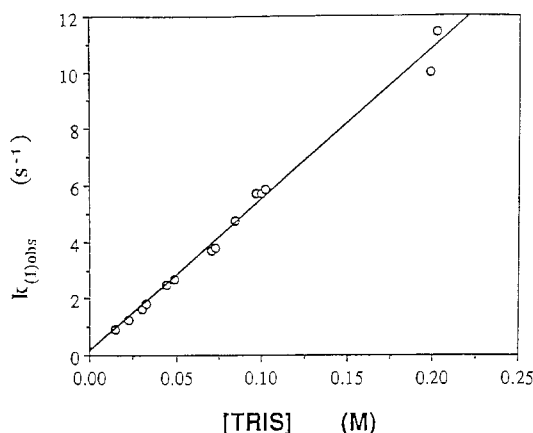
Figure 2. Plot of k_{\text{fast}} vs [TRIS] for reaction of \text{Cr}_2\text{O}_7^{2-} at 25 °C and I = 1.0 \text{ M} ( \text{NaClO}_4 ).
