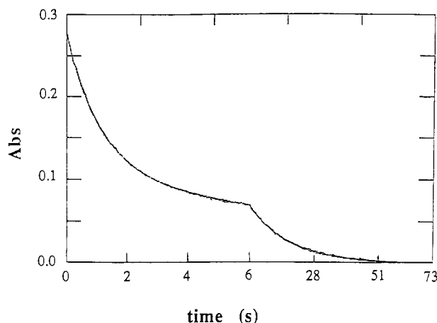
Figure 1. Variation of absorbance with time for the hydrolysis of \text{Cr}_2\text{O}_7^{2-} in the presence of TRIS buffer ( [\text{TRIS}]_{\text{T}} = 0.050 \text{ M} , [\text{Cr}]_{\text{T}} = 4 \times 10^{-3} \text{ M} , \lambda = 450 \text{ nm} , \text{pH} = 7.84 , 25^\circ\text{C} ). The data have been fitted to two consecutive first-order reactions with rate constants k_{\text{fast}} = 0.917 \text{ s}^{-1} and k_{\text{slow}} = 0.080 \text{ s}^{-1} , and the computed fit is superimposed on the experimental data. (Data were collected over two different time intervals: 0–6 and 6–73 s.)
